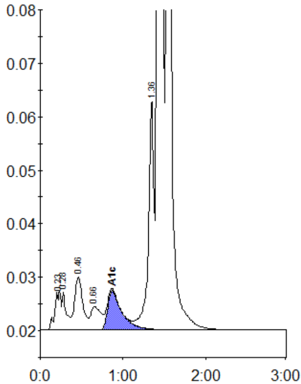
Peak table - ID: 10509947
